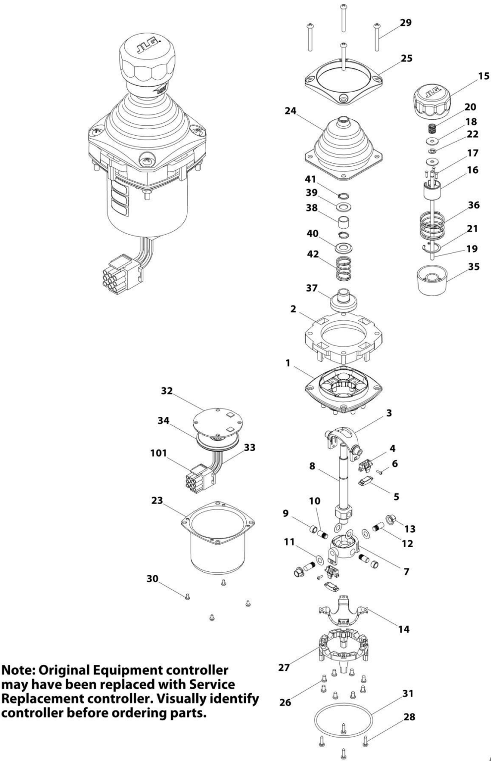
FIGURE 4-9. CONTROLLER ASSEMBLY (SWING AND LIFT) (SN 0300194240 through 0300211843)
