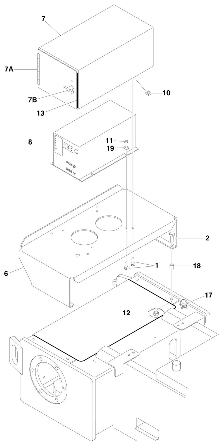
FIGURE 1-8. INVERTER INSTALLATION (OPTIONAL)
