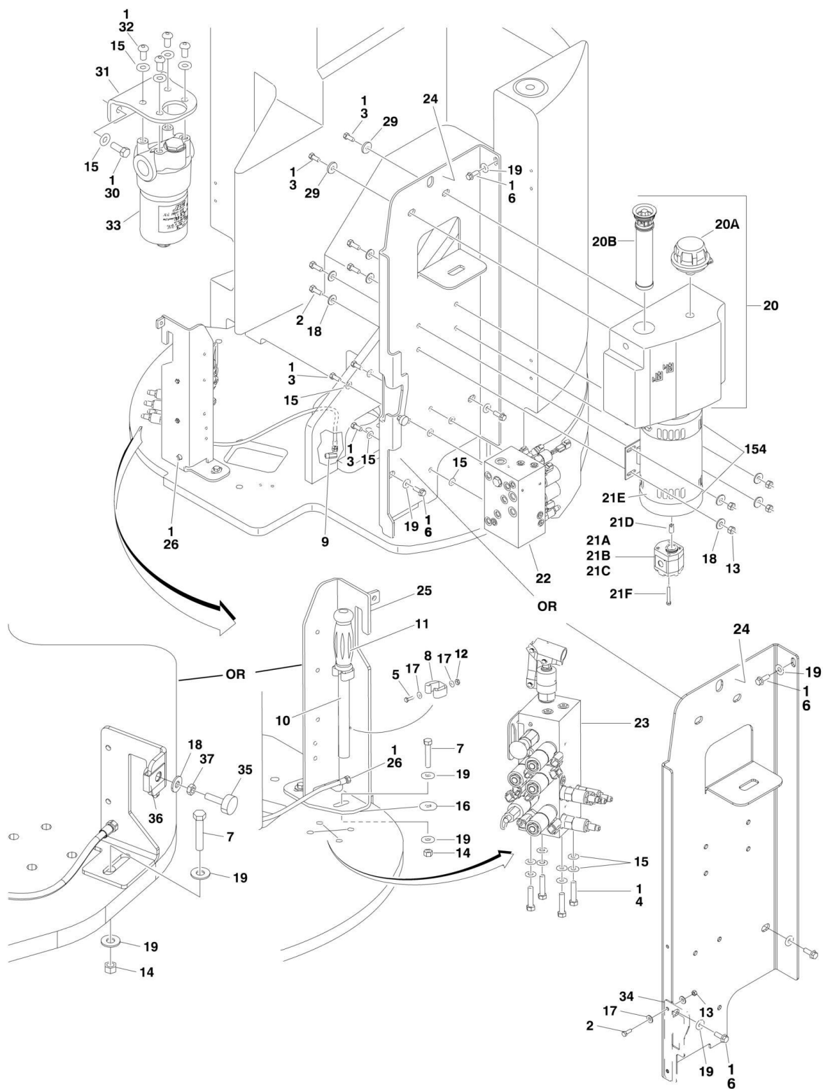
FIGURE 2-1. CONTROL VALVES AND TANK/MOTOR INSTALLATIONS
